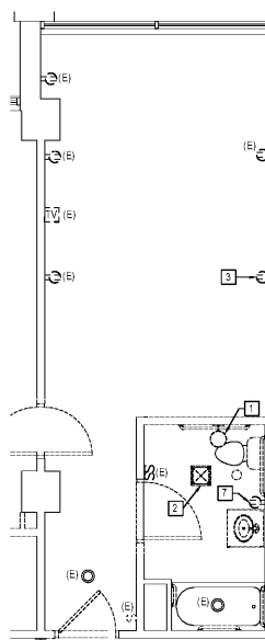
4 DEMOLITION PLAN - QQA1 E443 SCALE: 1/4" = 1'-0"
