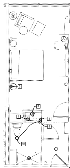
1 NEW WORK PLAN - KARI1 E443 SCALE: 1/4" = 1'-0"
