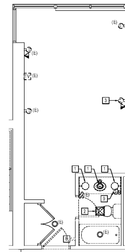
4 DEMOLITION PLAN - QQ3 E421 SCALE: 1/4" = 1'-0"
