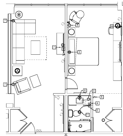
1 NEW WORK PLAN - KS1 E413 SCALE: 1/4" = 1'-0"
