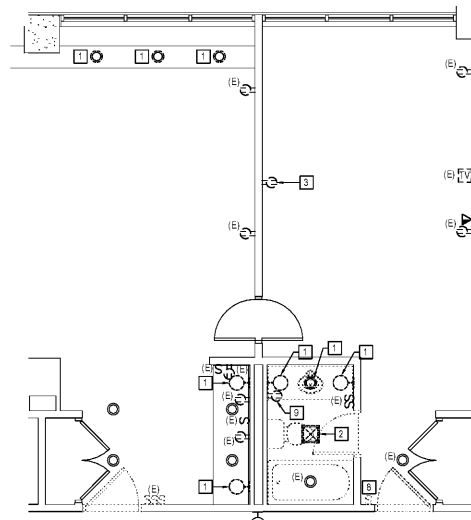
2 DEMOLITION PLAN - KS1 E413 SCALE: 1/4" = 1'-0"
