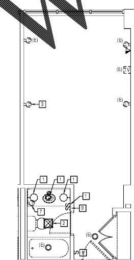
4 DEMOLITION PLAN - K1 E410 SCALE: 1/4" = 1'-0"
