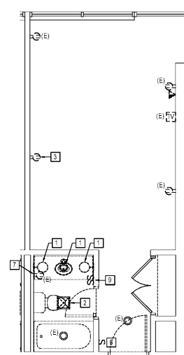
2 DEMOLITION PLAN - K2 E410 SCALE: 1/4" = 1'-0"
