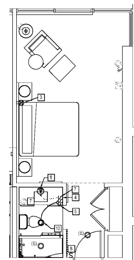
1 NEW WORK PLAN - K2 E410 SCALE: 1/4" = 1'-0"
