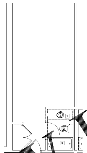
2 DEMOLITION PLAN - KA2-L R440 SCALE: 1/4" = 1'-0"
