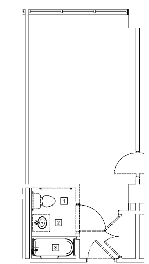
4 DEMOLITION PLAN - KA1I R440 SCALE: 1/4" = 1'-0"
