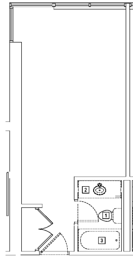
4 DEMOLITION PLAN - QQ3 P421 SCALE: 1/4" = 1'-0"
