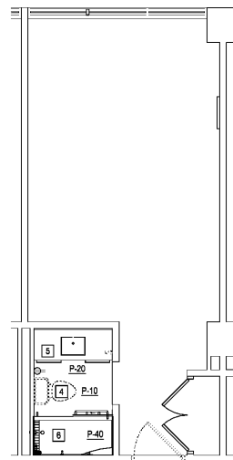
1 NEW WORK PLAN - K5 R412 SCALE: 1/4" = 1'-0"
