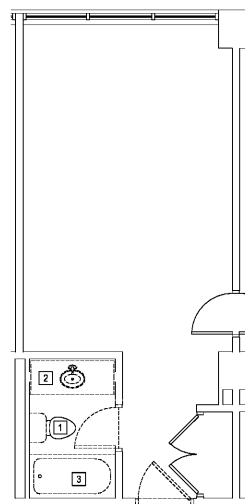
4 DEMOLITION PLAN - K3 P411 SCALE: 1/4" = 1'-0"
