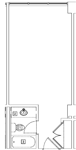
4 DEMOLITION PLAN - K1 P410 SCALE: 1/4" = 1'-0"
