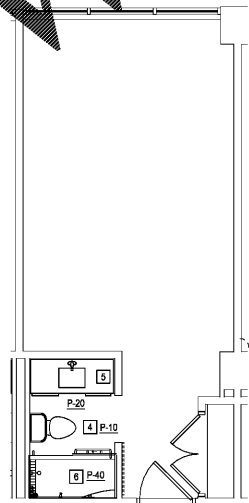
3 NEW WORK PLAN - K1 P410 SCALE: 1/4" = 1'-0"
