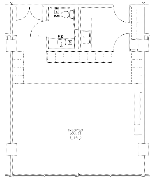
1 NEW WORK PLAN - EXECUTIVE LOUNGE P401 SCALE: 1/4" = 1'-0"
