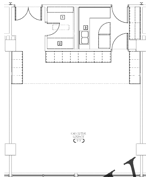
2 DEMOLITION PLAN - EXECUTIVE LOUNGE P401 SCALE: 1/4" = 1'-0"
