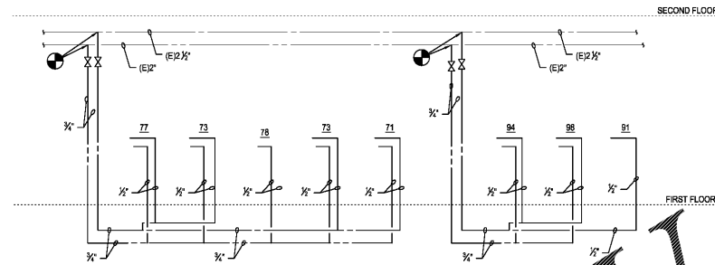
RISER DIAGRAM - DOMESTIC WATER - BAR SCALE: NONE
