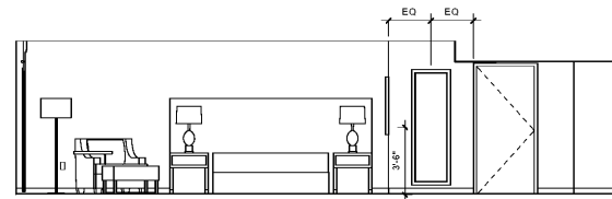
3E ELEVATION SCALE: 1/4" = 1'-0" DRAWING REF: A051
