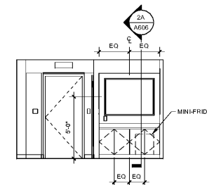
1A ELEVATION SCALE: 1/4" = 1'-0" DRAWING REF: A115
