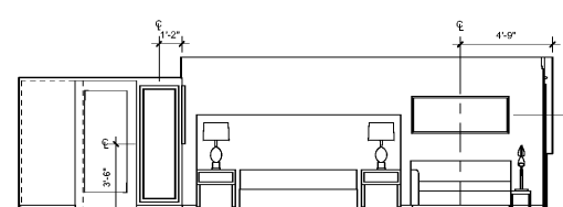
4B ELEVATION SCALE: 1/4" = 1'-0" DRAWING REF: A413
