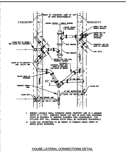
HOUSE LATERAL CONNECTIONS DETAIL
