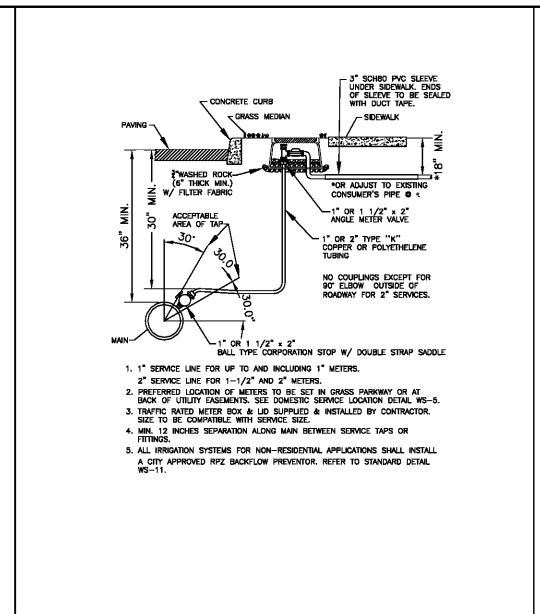
WATER SERVICES - 1" & 2" SINGLE SERVICE INSTALLATION
