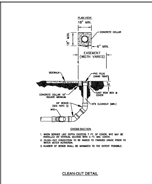
CLEAN-OUT DETAIL
