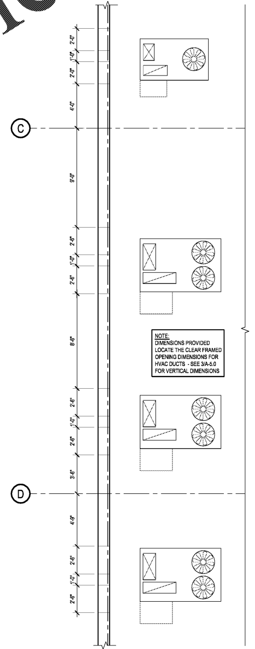
HVAC PENETRATION PLAN 2 SCALE: 1/4"=1'-0"
