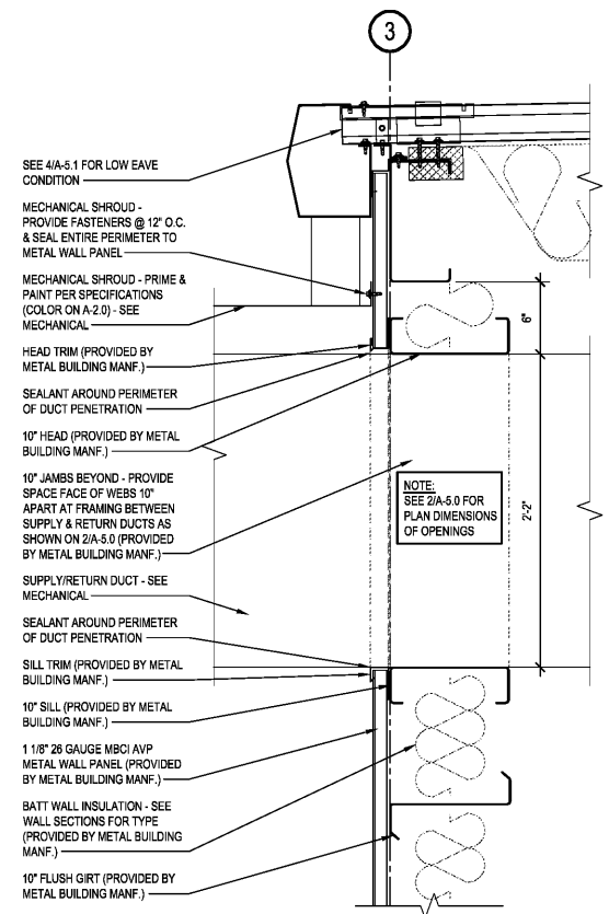
HVAC DUCT PENETRATION DETAIL 1 SCALE: 1 1/2"=1'-0"
