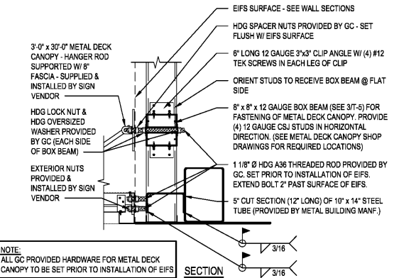
FRONT METAL DECK CANOPY ATTACHMENT DETAIL SCALE: 3/4"=1'-0"
