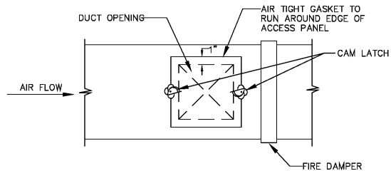
DUCT - TYPICAL NOT TO SCALE
