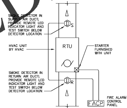
TYPICAL WIRING DIAGRAM - HVAC DUCT SMOKE DETECTOR NOT TO SCALE
