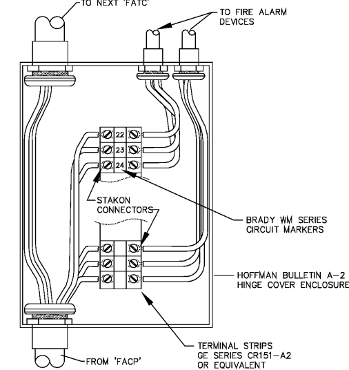
TYPICAL FIRE ALARM TERMINAL CABINET (FACT) NOT TO SCALE
