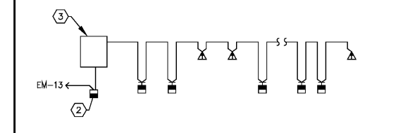
TYPICAL INTERCOM RISER DIAGRAM NOT TO SCALE
