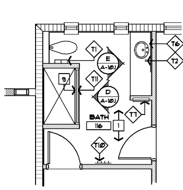
(C) ENLARGED FLOOR PLAN SCALE 1/4" = 1'-0"
