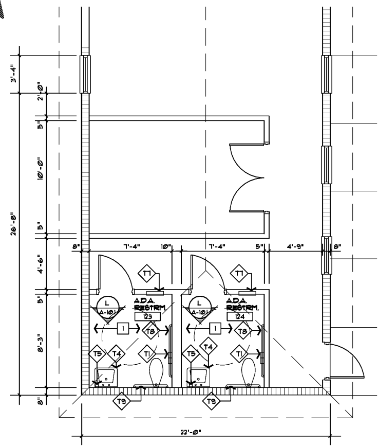
(C) ENLARGED FLOOR PLAN SCALE 1/4" = 1'-0"
