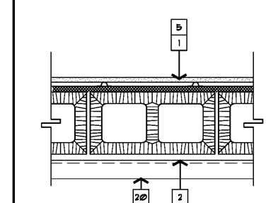
W-1 WALL TYPE SCALE 1/2" = 1'-0"
