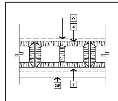
W-3 WALL TYPE SCALE 1/2" = 1'-0"
