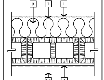
W-6 WALL TYPE SCALE 1/2" = 1'-0"
