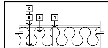
P-3A - 1 HR. RATED U486 PART. TYPE SCALE 1/2" = 1'-0"
