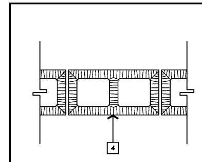
W-2 WALL TYPE SCALE 1/2" = 1'-0"
