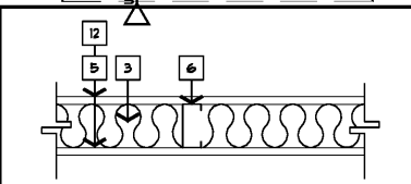
P-2A - 1 HR. RATED U486 PART. TYPE SCALE 1/2" = 1'-0"
