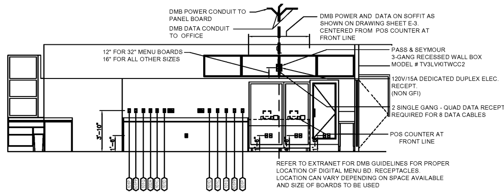
DUNKIN' DONUTS – SERVICE AREA ELEVATION NO SCALE
