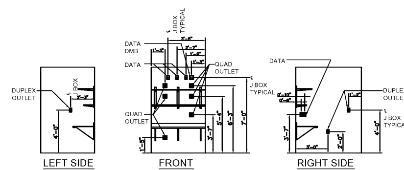
DUNKIN' DONUTS – MANAGER'S OFFICE ELEVATION NO SCALE
