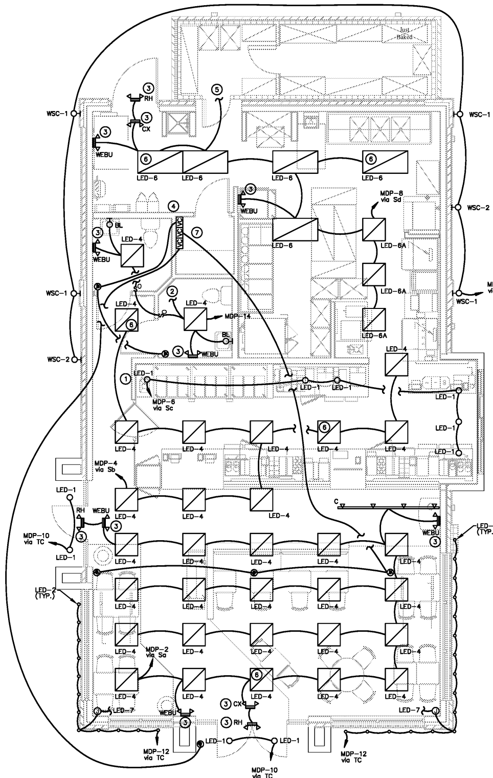
ELECTRICAL LIGHTING PLAN SCALE: 1/4" = 1'-0"
