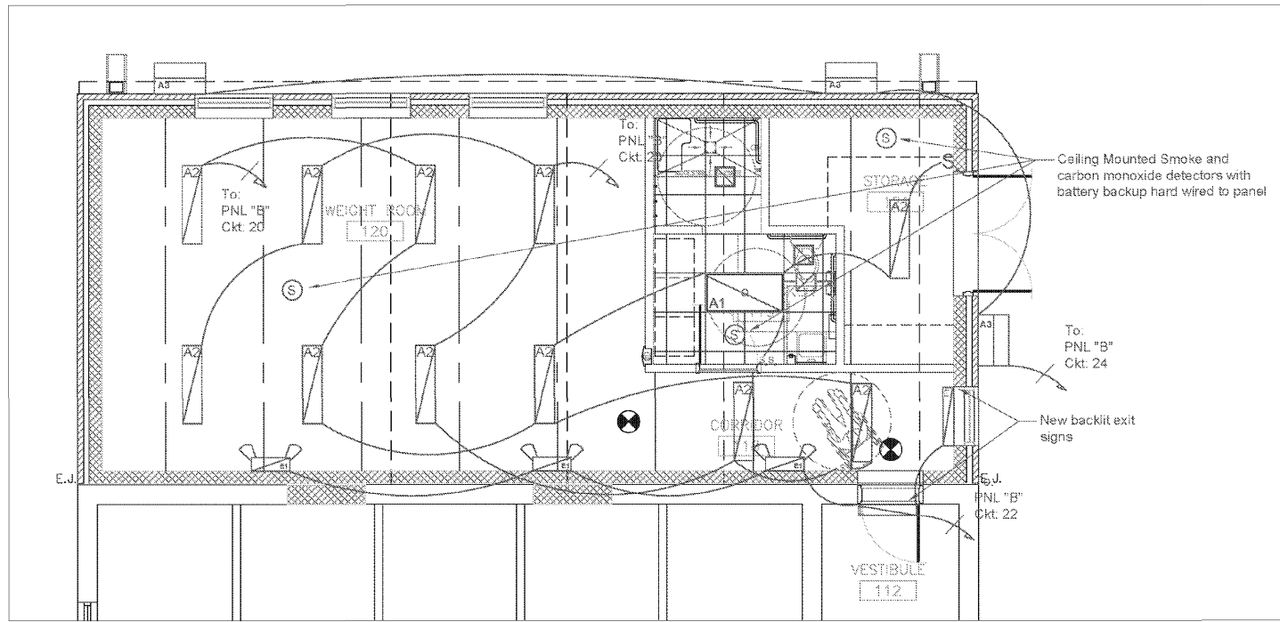
2 E1.1 Lighting Install Plan Scale: 1/4" = 1' - 0"
