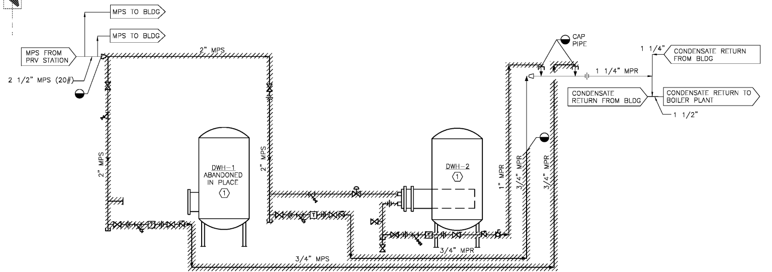
B BLDG 9 DOMESTIC WATER HEATERS STEAM AND CONDENSATE DEMOLITION DIAGRAM NO SCALE
