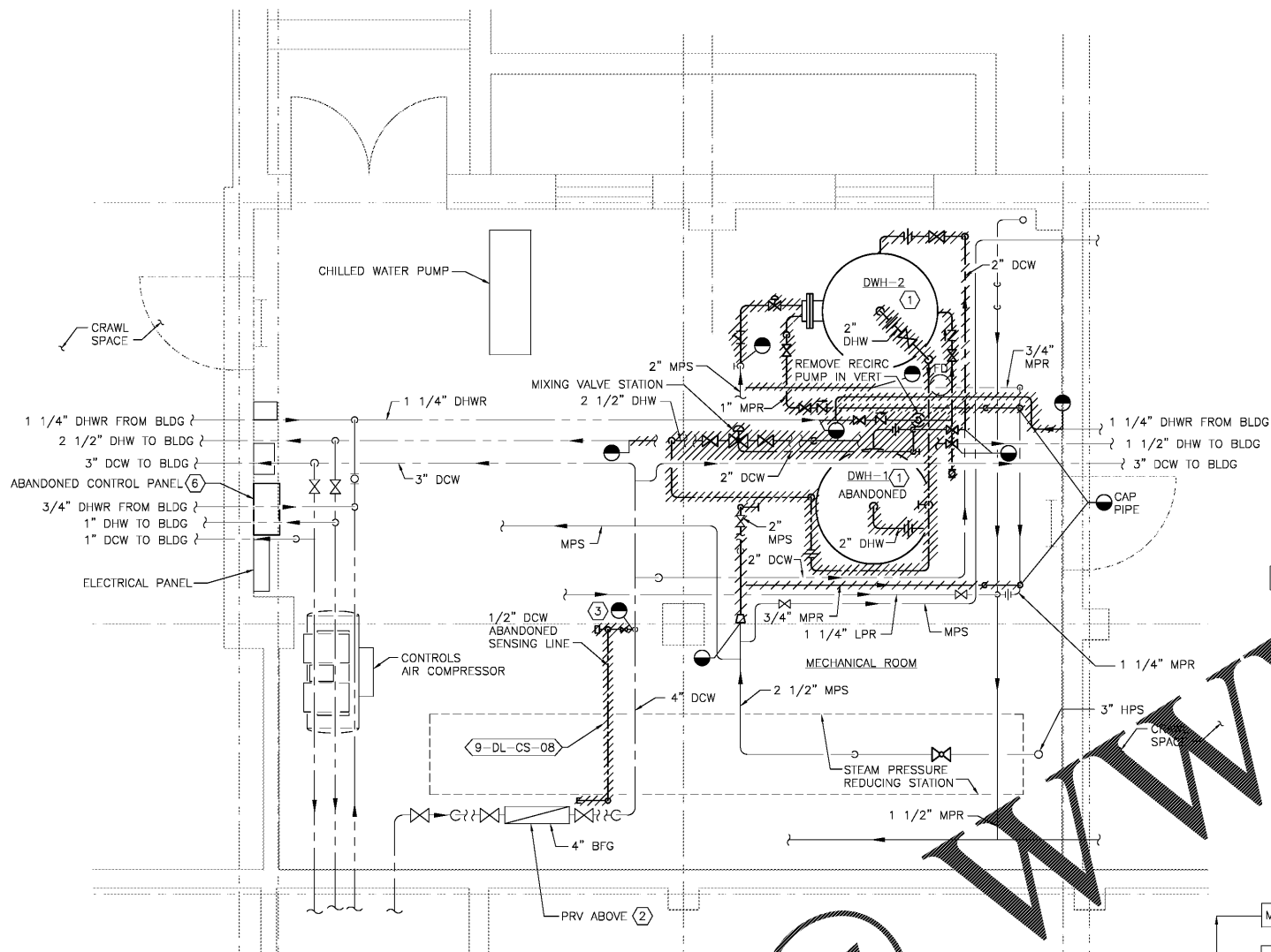
PLAN NORTH 1 ENLARGED SUB-BASEMENT PLUMBING DEMOLITION PLAN SCALE: 1/2" = 1'-0"
