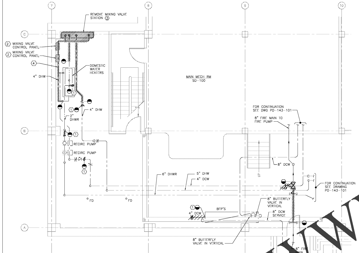
PLAN NORTH ① ENLARGED SUB-BASEMENT PLUMBING PLAN SCALE: 1/4" = 1'-0"
