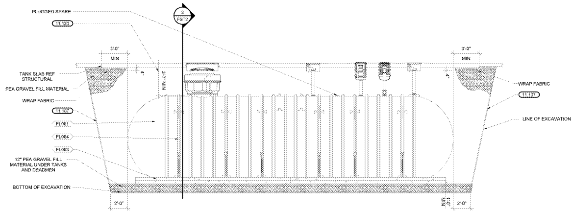
1 UNDERGROUND STORAGE TANK DETAIL 1/8" = 1'-0"
