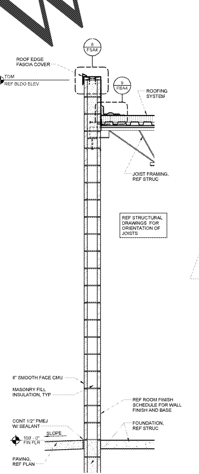
9 WALL SECTION 3/4" x 1'-0"
