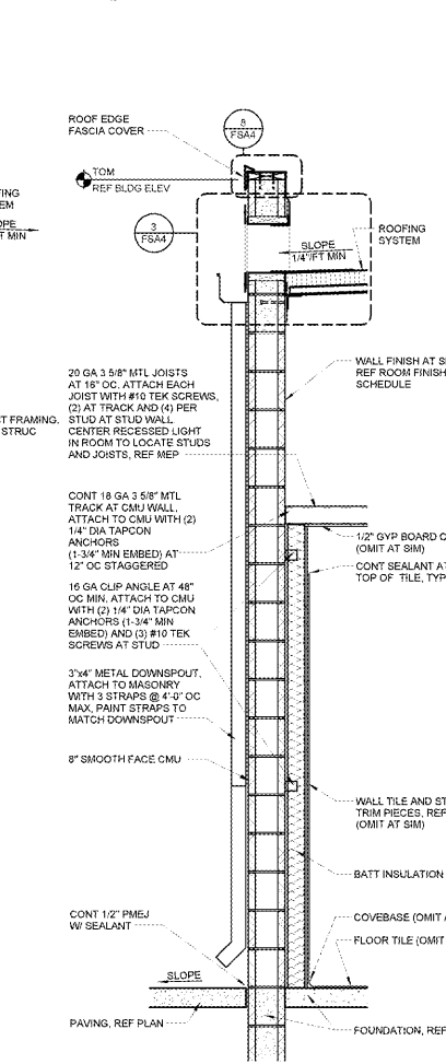
1 WALL SECTION 3/4" x 1'-0"
