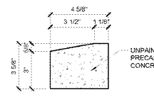
11 PRECAST CONC WATER TABLE 3' x 1'-0"
