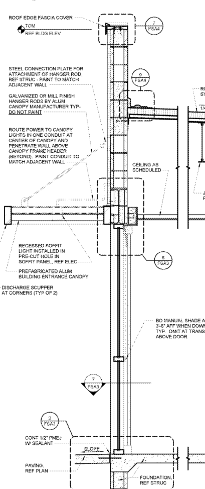
5 WALL SECTION 3/4" x 1'-0"
