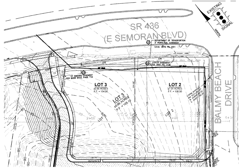
PLAN VIEW
