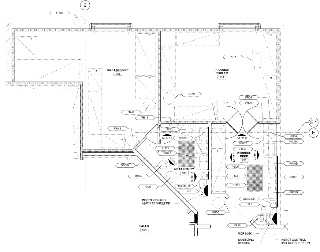
1 ENLARGED PRODUCE PREP FIXTURE PLAN 1/4" = 1'-0"
