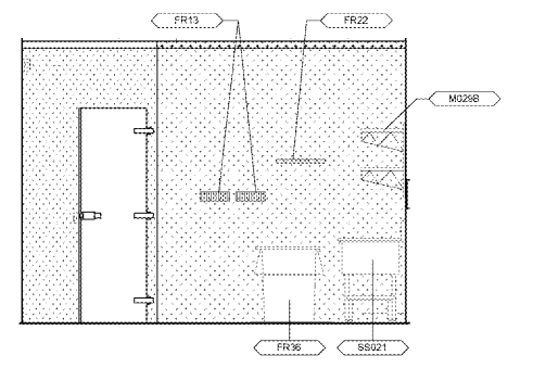
5 MEAT UTILITY ELEVATION 3/8" = 1'-0"
