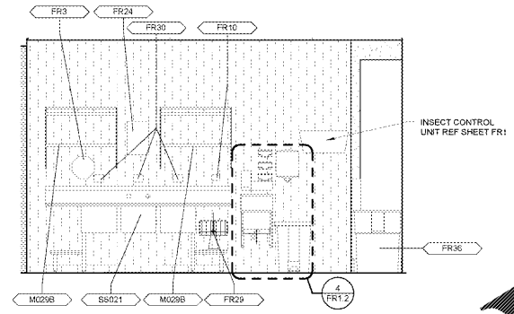
6 MEAT UTILITY ELEVATION 3/8" = 1'-0"
