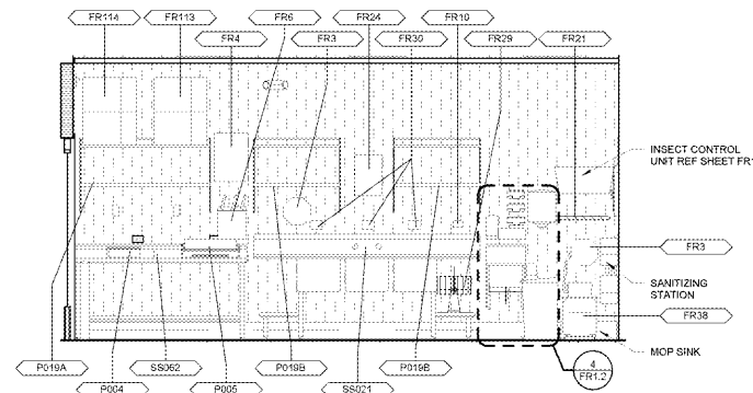
2 PRODUCE PREP ELEVATION 3/8" = 1'-0"
