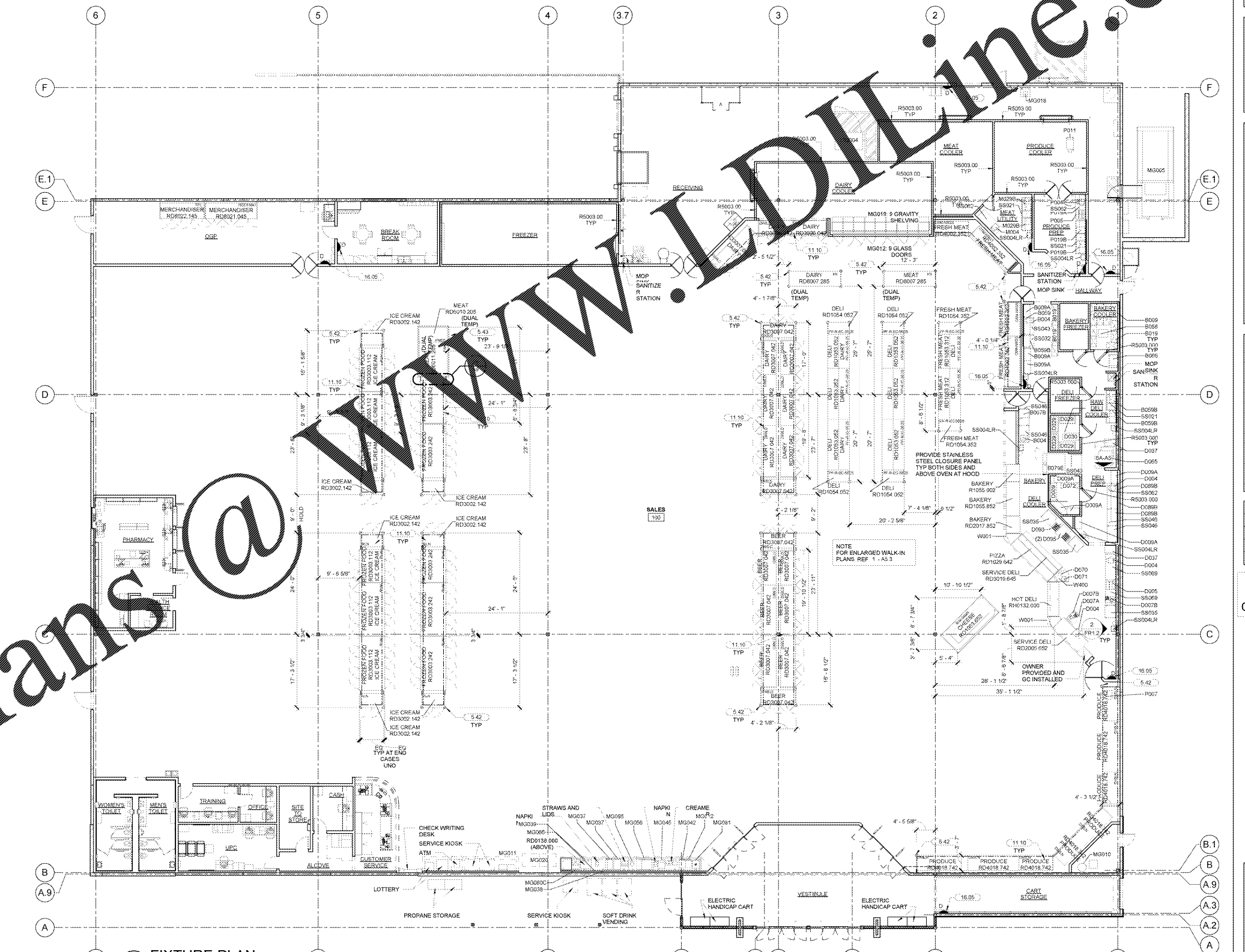
1 FIXTURE PLAN 1" = 10'-0"
