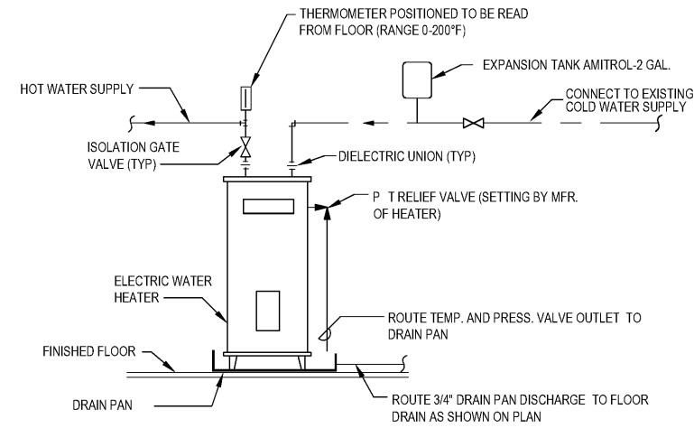
1 ELECTRIC WATER HEATER DETAIL SCALE: NONE
