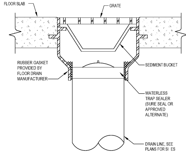
2 FLOOR DRAIN TRAP SEAL DETAIL SCALE: NONE
