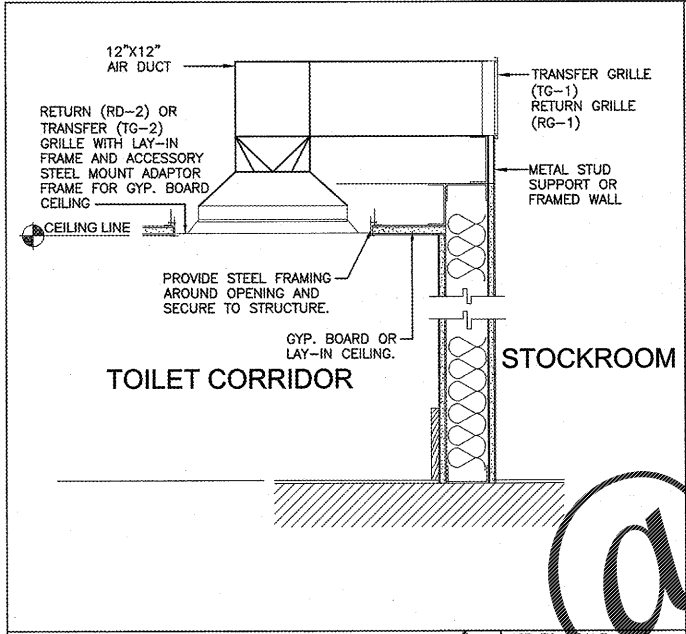
TRANSFER/RETURN AIR GRILLE DETAIL
