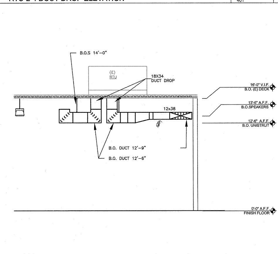
RTU-1 DUCT DROP ELEVATION
