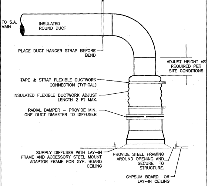
DIFFUSER MOUNTING DETAIL
