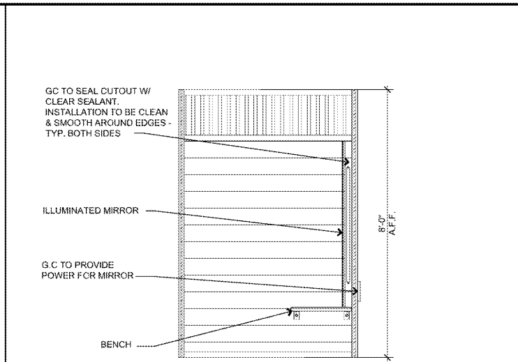
FITTING ROOM ELEVATION SCALE: 1/2" = 1'-0" 6
