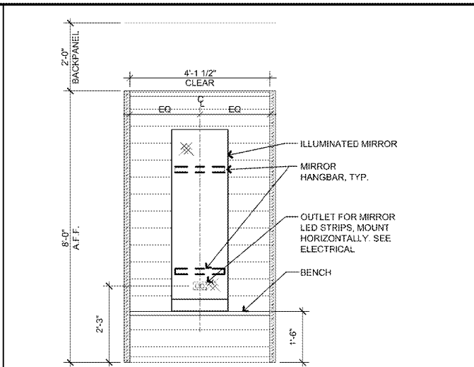
FITTING ROOM ELEVATION SCALE: 1/2" = 1'-0" 9
