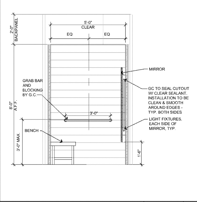
HC FITTING ROOM ELEVATION SCALE: 1/2" = 1'-0" 11
