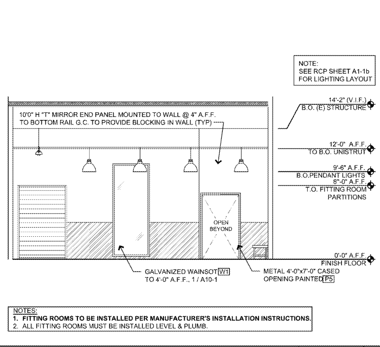
FITTING ROOM ELEVATION SCALE: 3/16" = 1'-0" 1
