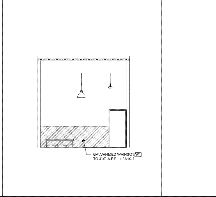
FITTING ROOM ELEVATION SCALE: 3/16" = 1'-0" 4
