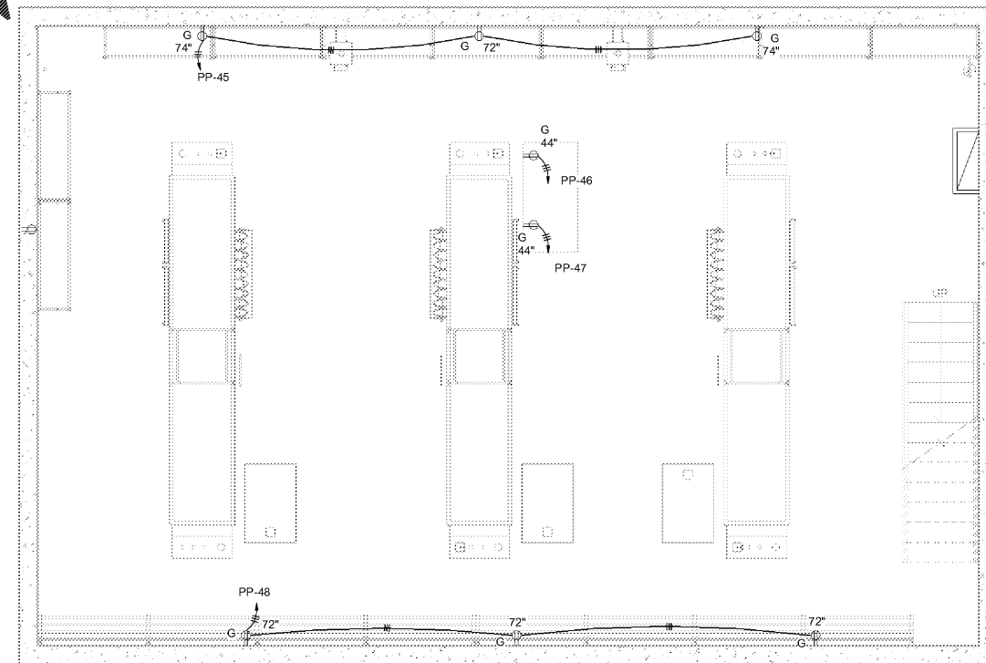
② POWER & AUXILIARY PIT FLOOR PLAN 1/4" = 1'-0"
