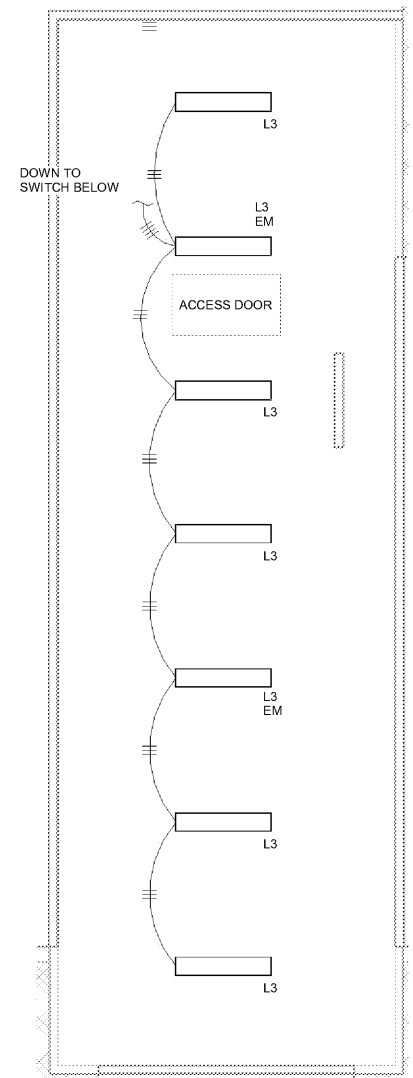
④ LIGHTING MEZZ FLOOR PLAN 1/4" = 1'-0"
