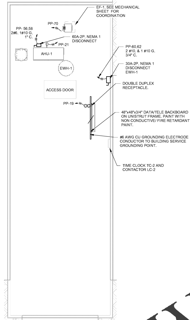
③ POWER & AUXILIARY MEZZ FLOOR PLAN 1/4" = 1'-0"
