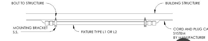
② FIXTURE L1 AND L2 MOUNTING DETAIL 1" = 1'-0"
