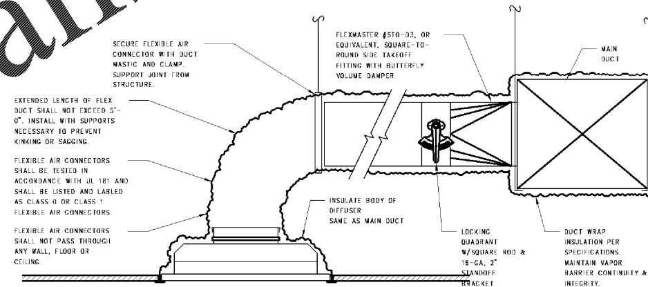
FLEXIBLE AIR CONNECTION DETAIL
