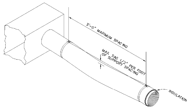
FLEX DUCT SUPPORT DETAIL
