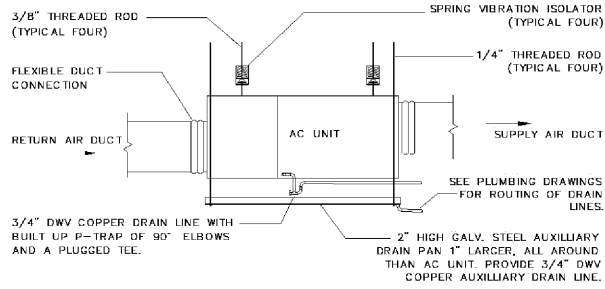
AIR HANDLER HANGING DETAIL
