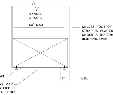
DUCT SUPPORT DETAILS
