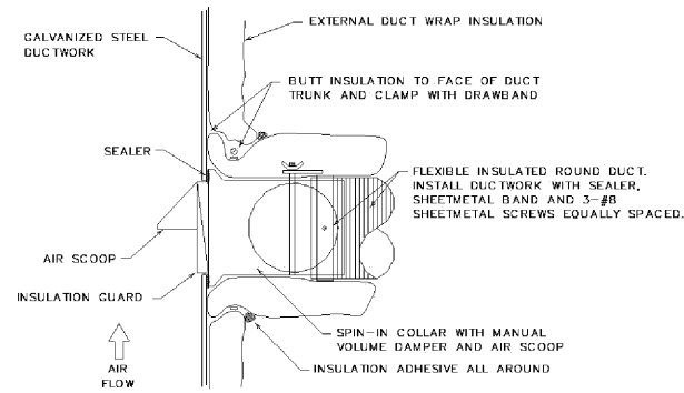
ROUND DUCT SPIN-IN DETAIL
