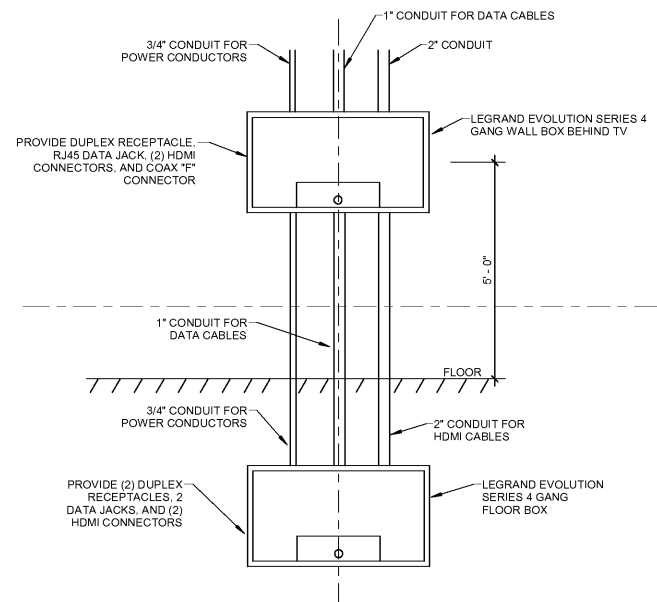
1 TV WALL CONFERENCE ROOM DETAIL E004 NOT TO SCALE
