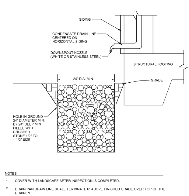
6 L-3 INSTALLATION DETAIL M003 NOT TO SCALE
