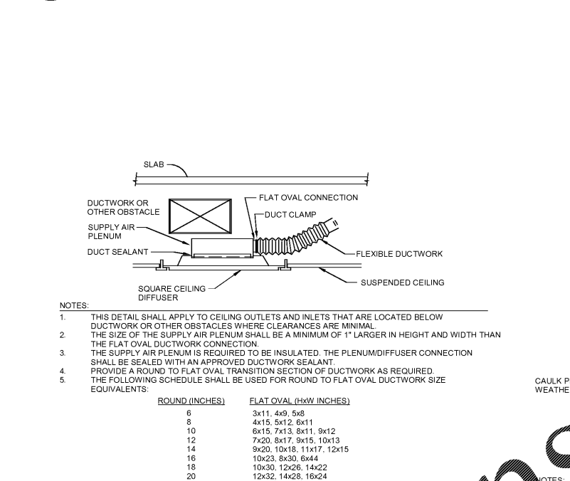
3 L-1 INSTALLATION DETAIL M003 NOT TO SCALE
