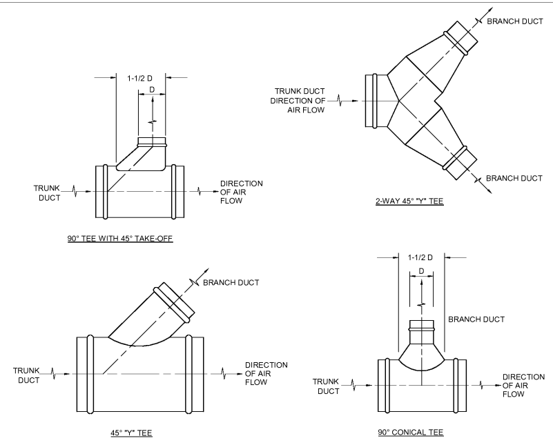
1 ROUND DUCT BRANCH TAKE OFF DETAIL M003 NOT TO SCALE
