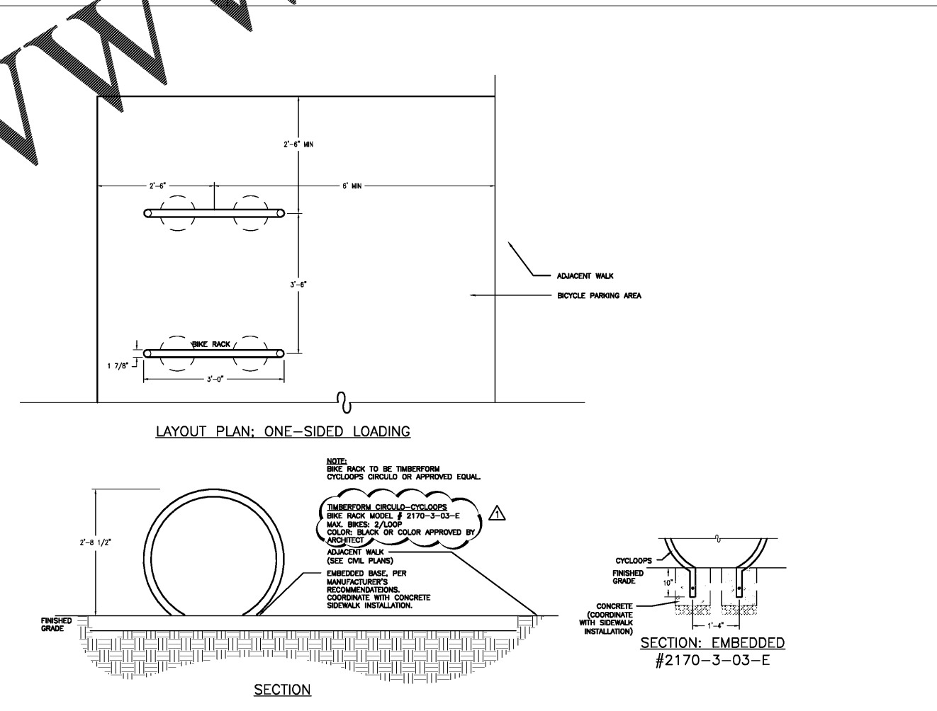
A2 BICYCLE RACK LOOP DETAIL NOT TO SCALE L200
