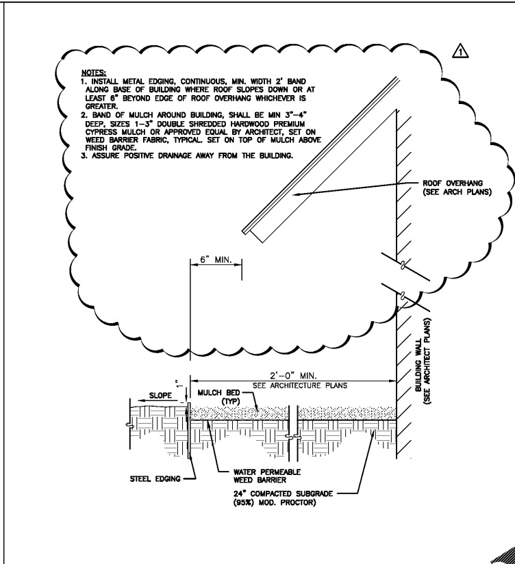
B2 MULCH BAND DETAIL NOT TO SCALE L200
