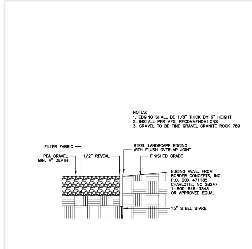
B1 PEAS GRAVEL WITH STEEL EDGE DETAIL NOT TO SCALE L200
