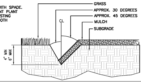
A1 TRENCH EDGE DETAIL NOT TO SCALE L200
