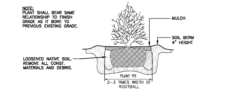
B1 SHRUB PLANTING DETAIL NOT TO SCALE L200
