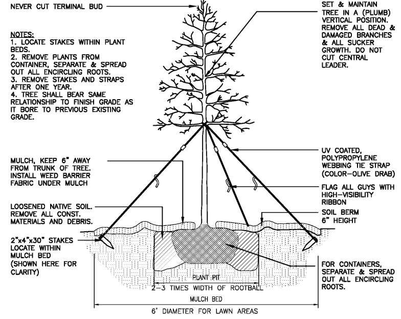
C1 TREE PLANTING DETAIL NOT TO SCALE L200
