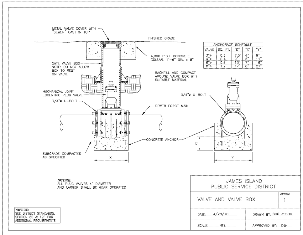
A VALVE AND VALVE BOX
