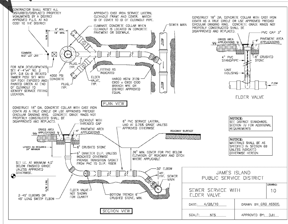
D SANITARY SEWER SERVICE
