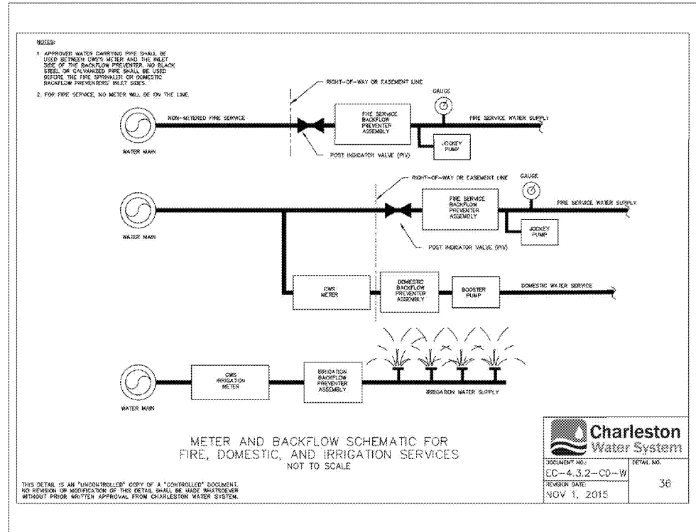
D METER AND BACKFLOW FOR SERVICES
