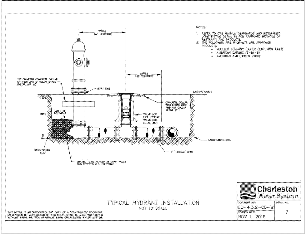
A FIRE HYDRANT INSTALLATION
