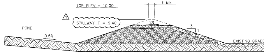
SPILLWAY ELEVATION
