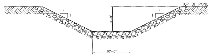
SPILLWAY SECTION
